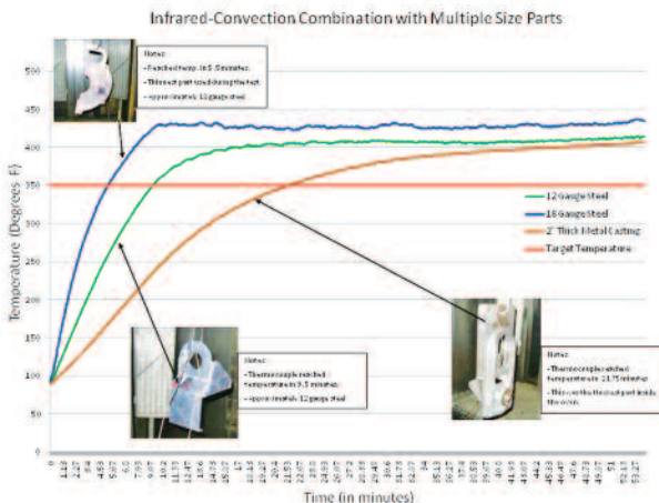
Temperature profiles for multiple-size parts
